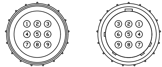
CPC CONNECTOR BACK VIEW- WIRE INSERTION FRONT VIEW
