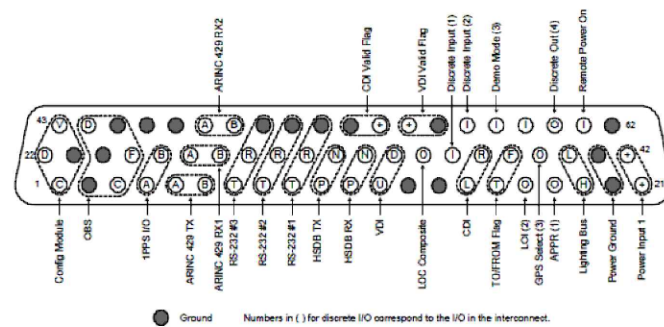
Figure 5-2 J1751 62-Pin Connector View Rear of Unit
