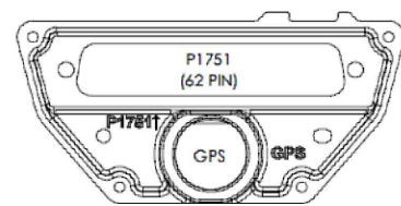
Figure 5-1 GPS 175 Rear Connector Layout
