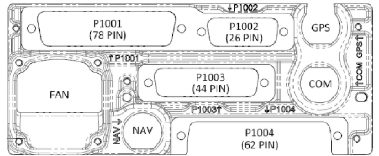
Figure A-12. GTN 6XX Connector Layout Detail—Rear View
